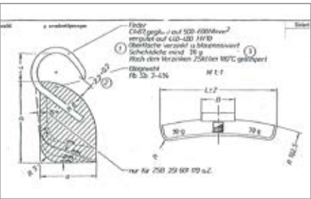
Technical drawing of a knock-on weight
